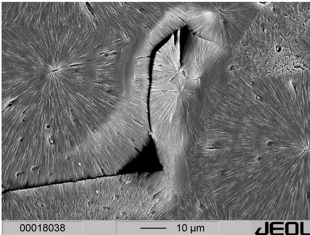
inter-pherulitic cracks in PHB SEM picture
